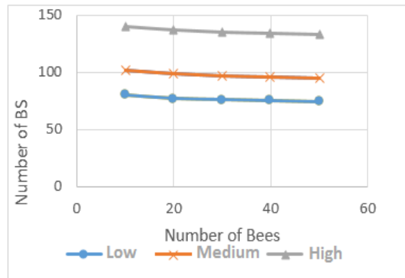
Fig. 16. Optimization results dependence (number of BS) on the number of bees for MS of different capacity
